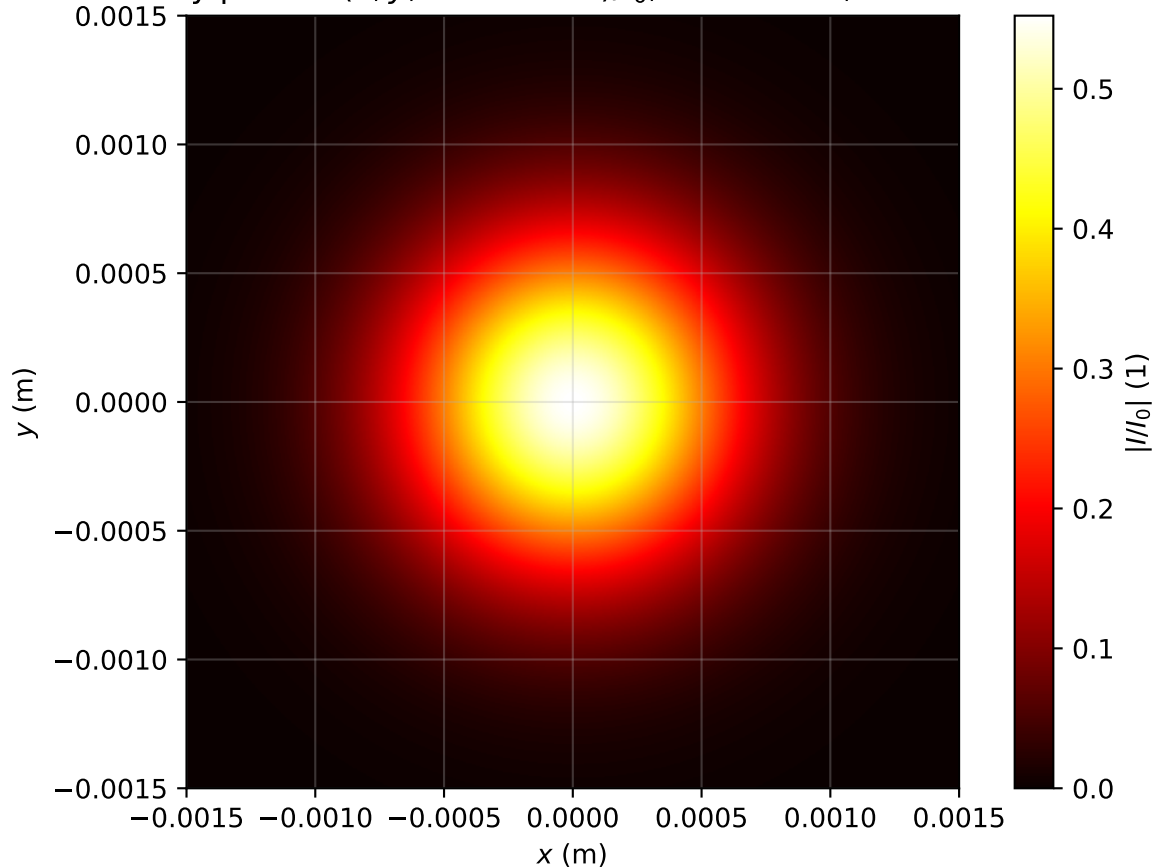
Intensity profile I(x, y, z = 2.149m)/I_0 , P_{in}=0.2P_{cr} , artificial time
